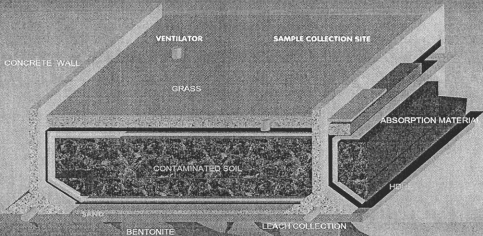
Figure 1. The model of active landfill bioreactor
